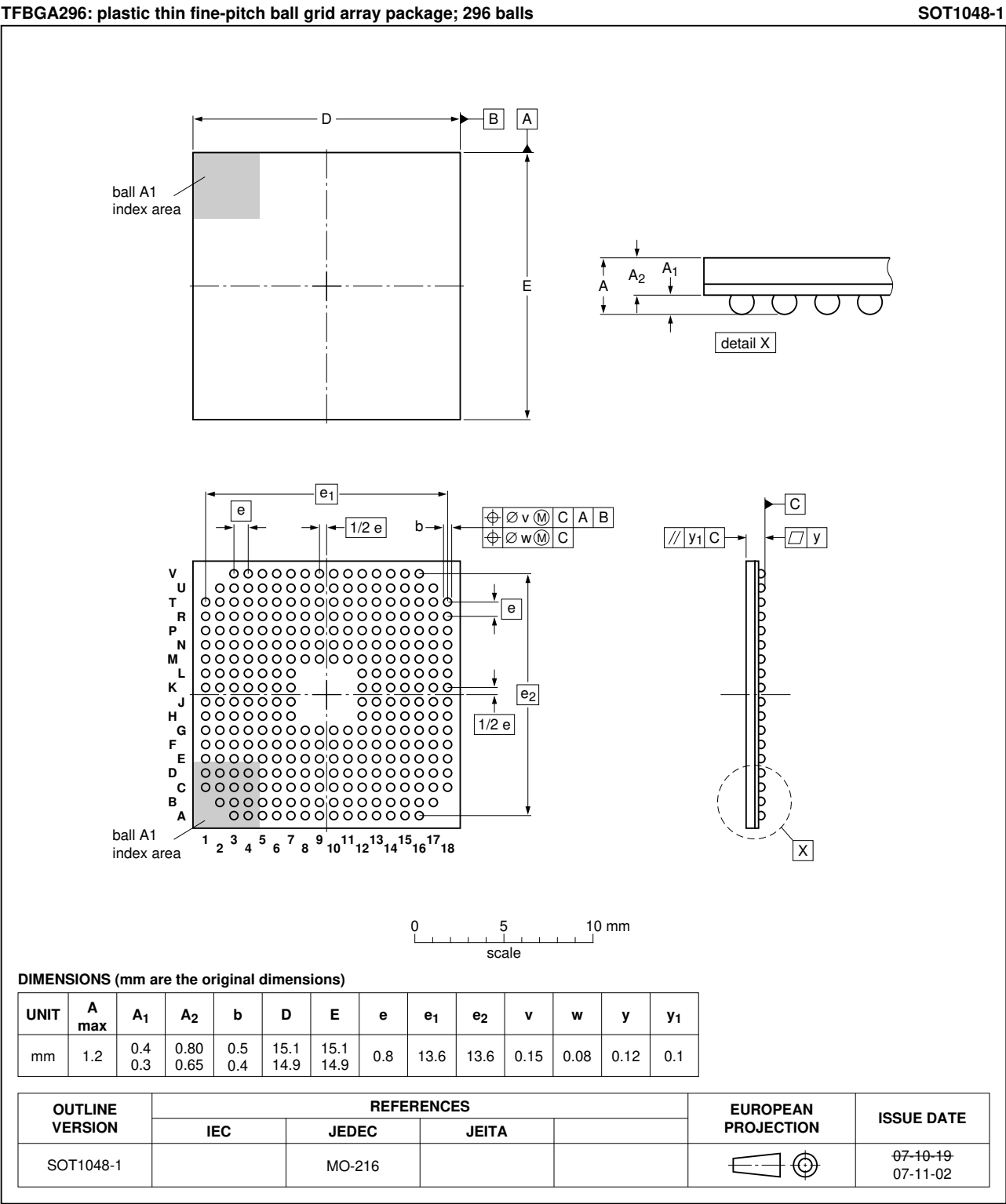
Fig 25. Package outline SOT1048-1 (TFBGA296)
