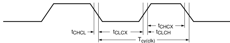
Fig 13. External clock timing (with an amplitude of at least V_{i(RMS)} = 200\text{ mV} )
