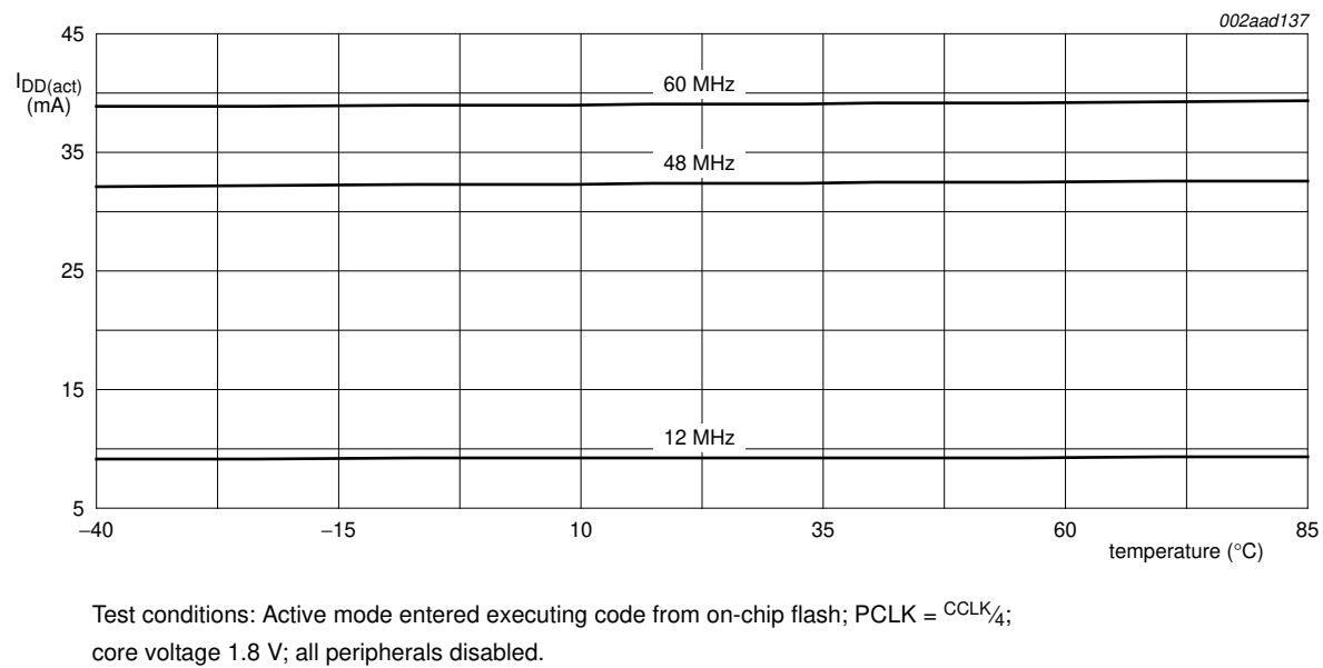
Fig 15. Typical LPC2109/01, LPC2119/01, and LPC2129/01 I_{DD(act)} measured at different temperatures
