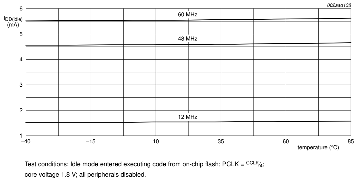
Fig 16. Typical LPC2109/01, LPC2119/01, and LPC2129/01 I_{DD(idle)} measured at different temperatures
