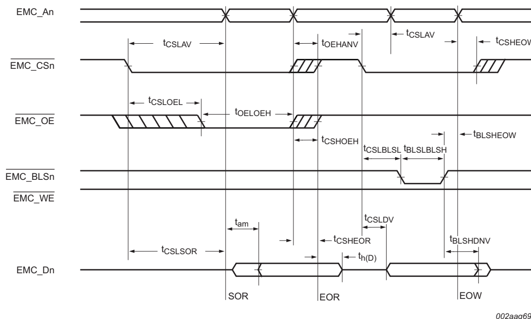
Fig 32. External static memory read/write access (PB = 0)
