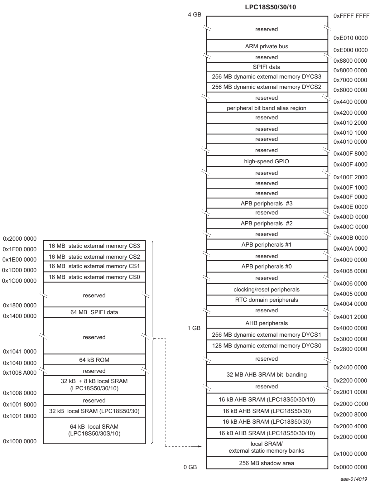
Fig 7. LPC18S50/S30/S10 Memory mapping (overview)
