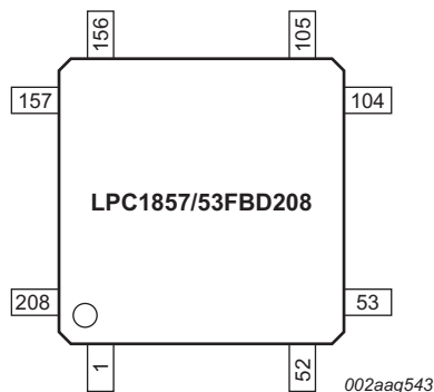
Fig 4. Pin configuration LQFP208 package
