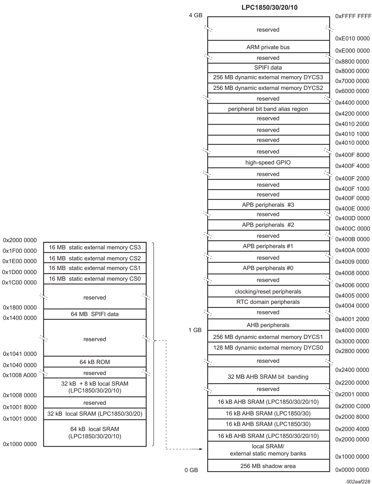
Fig 7. LPC1850/30/20/10 Memory mapping (overview)
