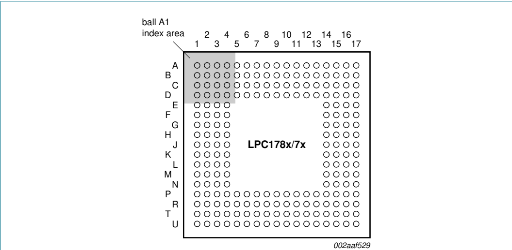
Fig 3. Pin configuration (TFBGA208)
