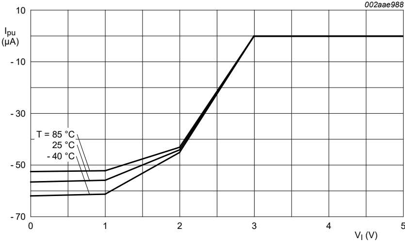
Figure 19. Typical pull-up current I_{pu} versus input voltage V_I
