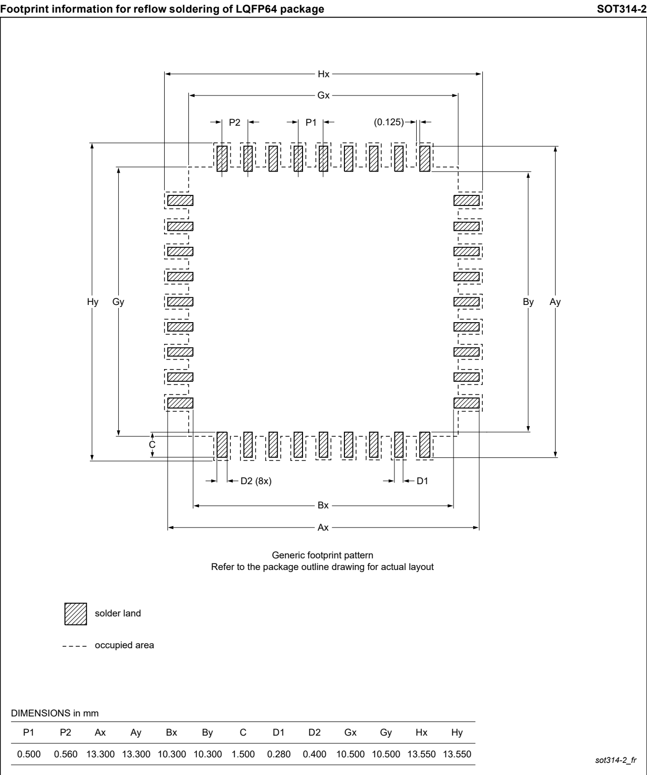
Figure 43. Reflow soldering for the LQFP64 package
