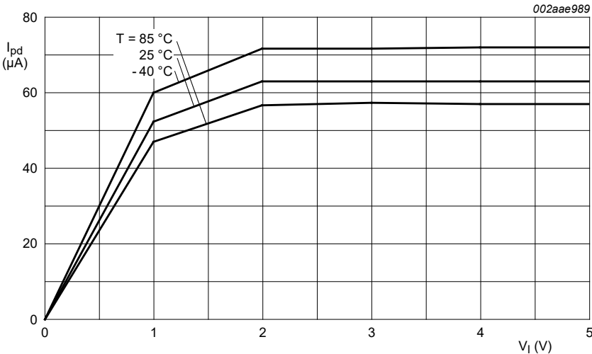
Figure 20. Typical pull-down current I_{pd} versus input voltage V_I
