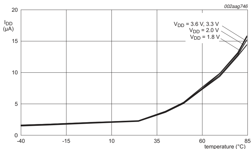
Fig 12. Typical supply current versus temperature in Power-down mode
