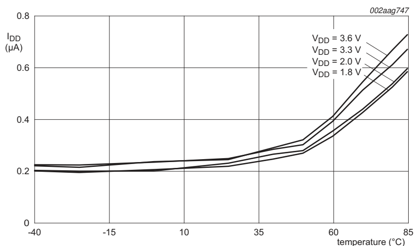
Fig 13. Typical supply current versus temperature in Deep power-down mode
