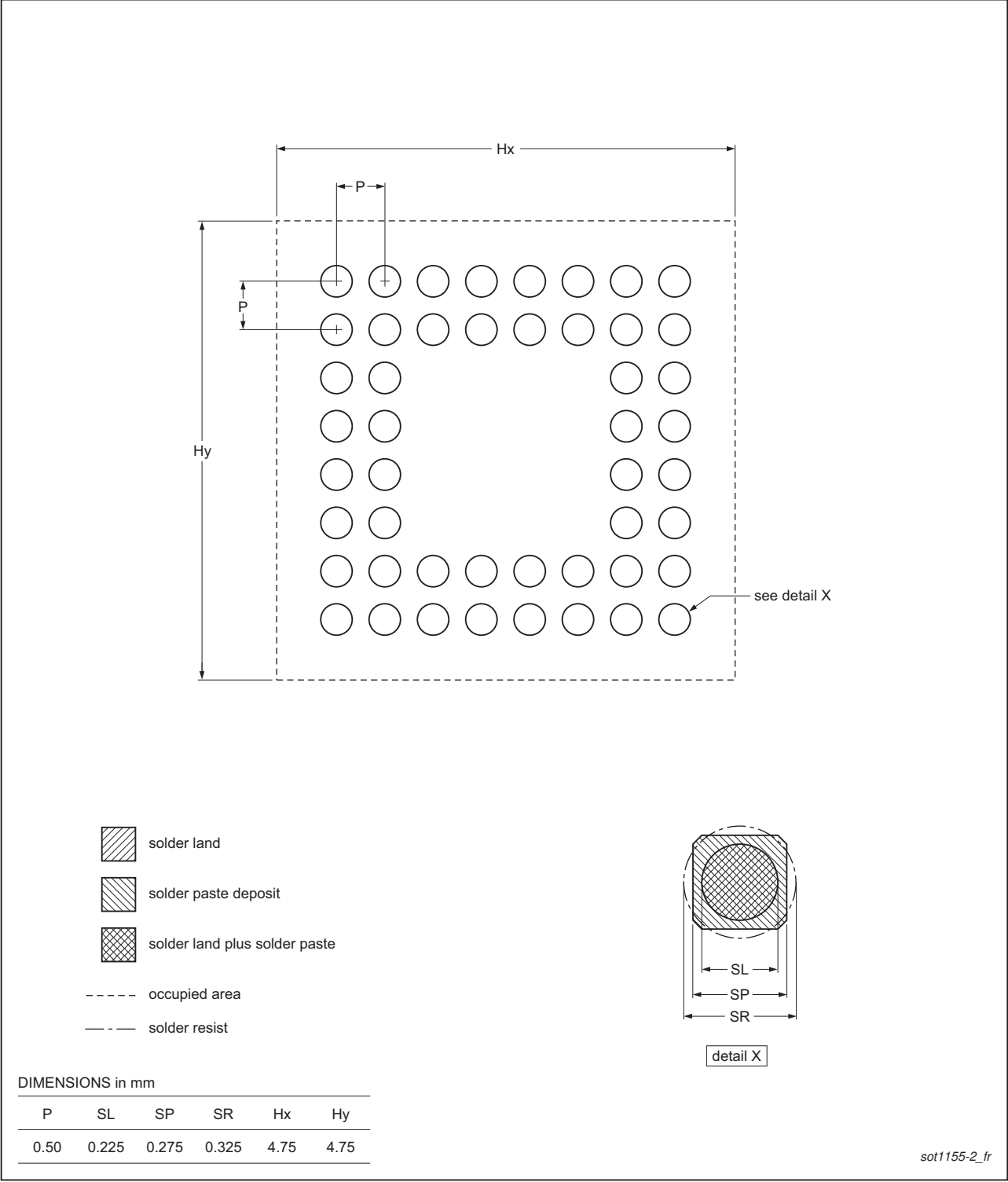
Fig 70. Reflow soldering for the TFBGA48 package
