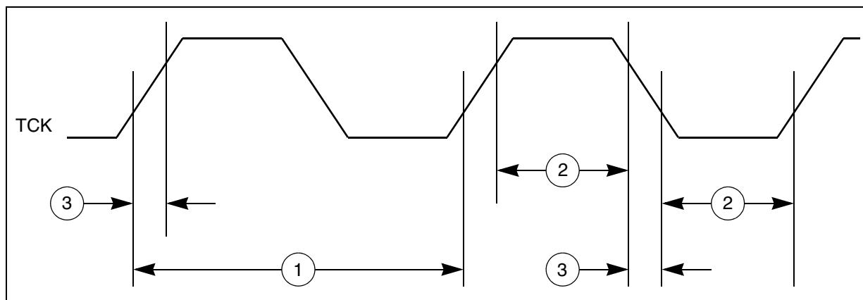
Figure 32. JTAG test clock input timing
