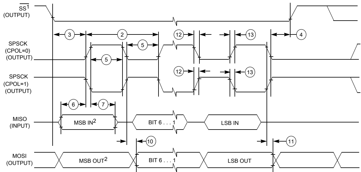
Figure 19. LPSPi master mode timing (CPHA = 0)
