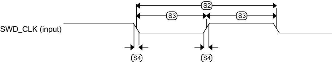
Figure 30. Serial wire clock input timing
