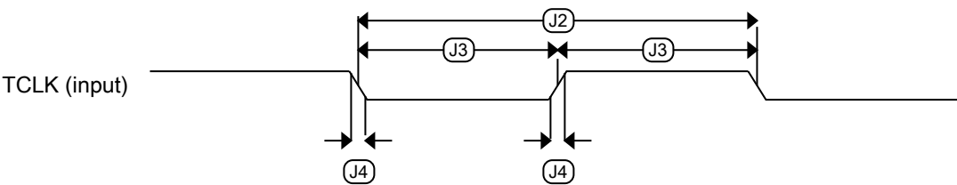
Figure 33. Test clock input timing
