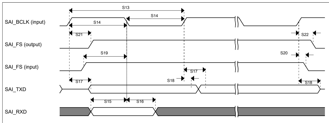
Figure 24. SAI Timing — Slave modes
