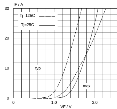
Fig.11. Damper forward characteristic I_F = f(V_F) ; parameter T_J
