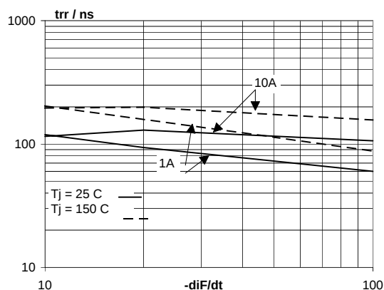
Fig.9. Modulator maximum t_{rr} measured to 25% of I_{rm} ; T_j = 25^\circ\text{C} and 150^\circ\text{C}
