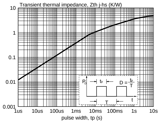
Fig.9. Transient thermal impedance Z_{th} = f(t_p)
