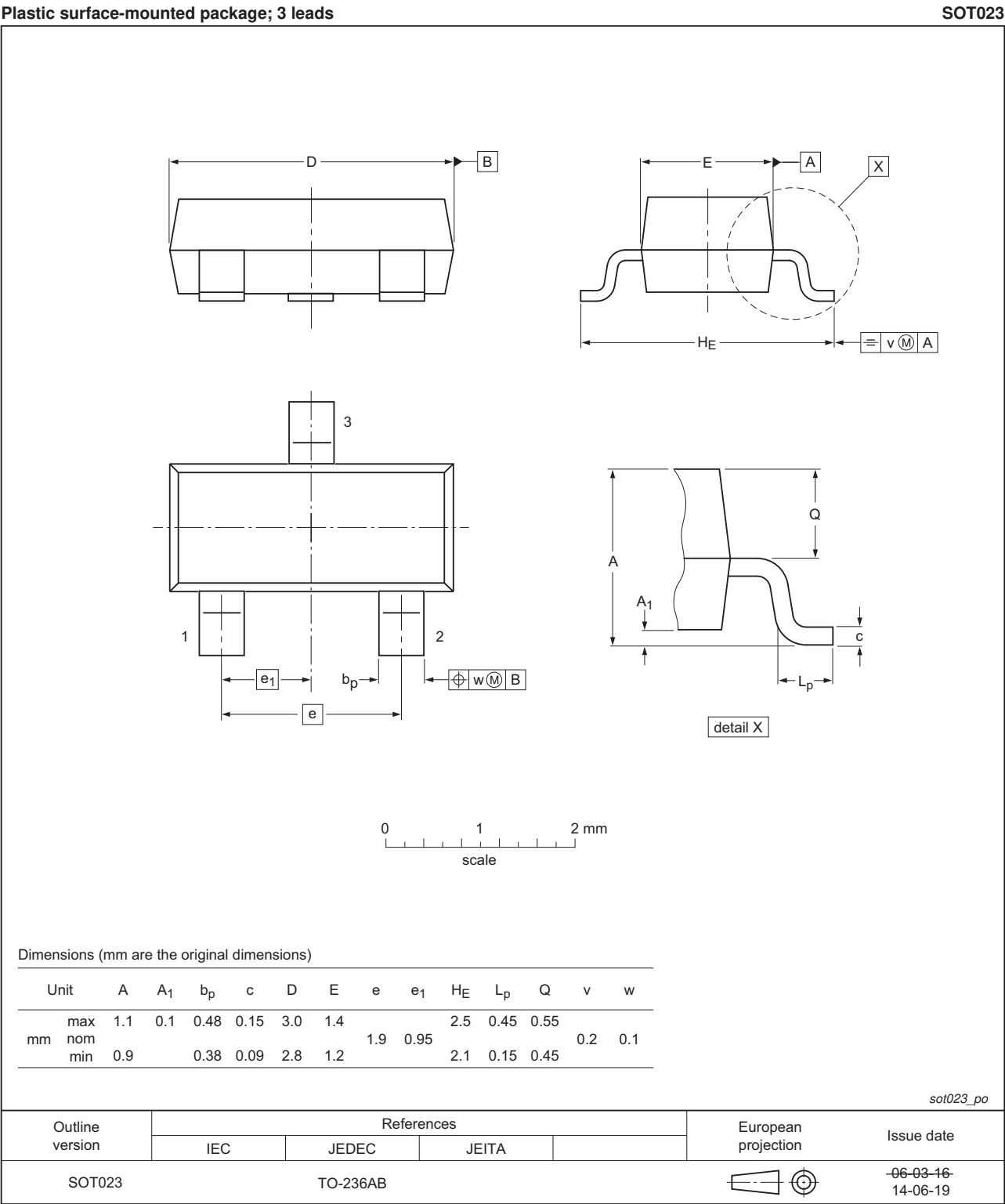
Fig 4. Package outline SOT23 (TO-236AB)
