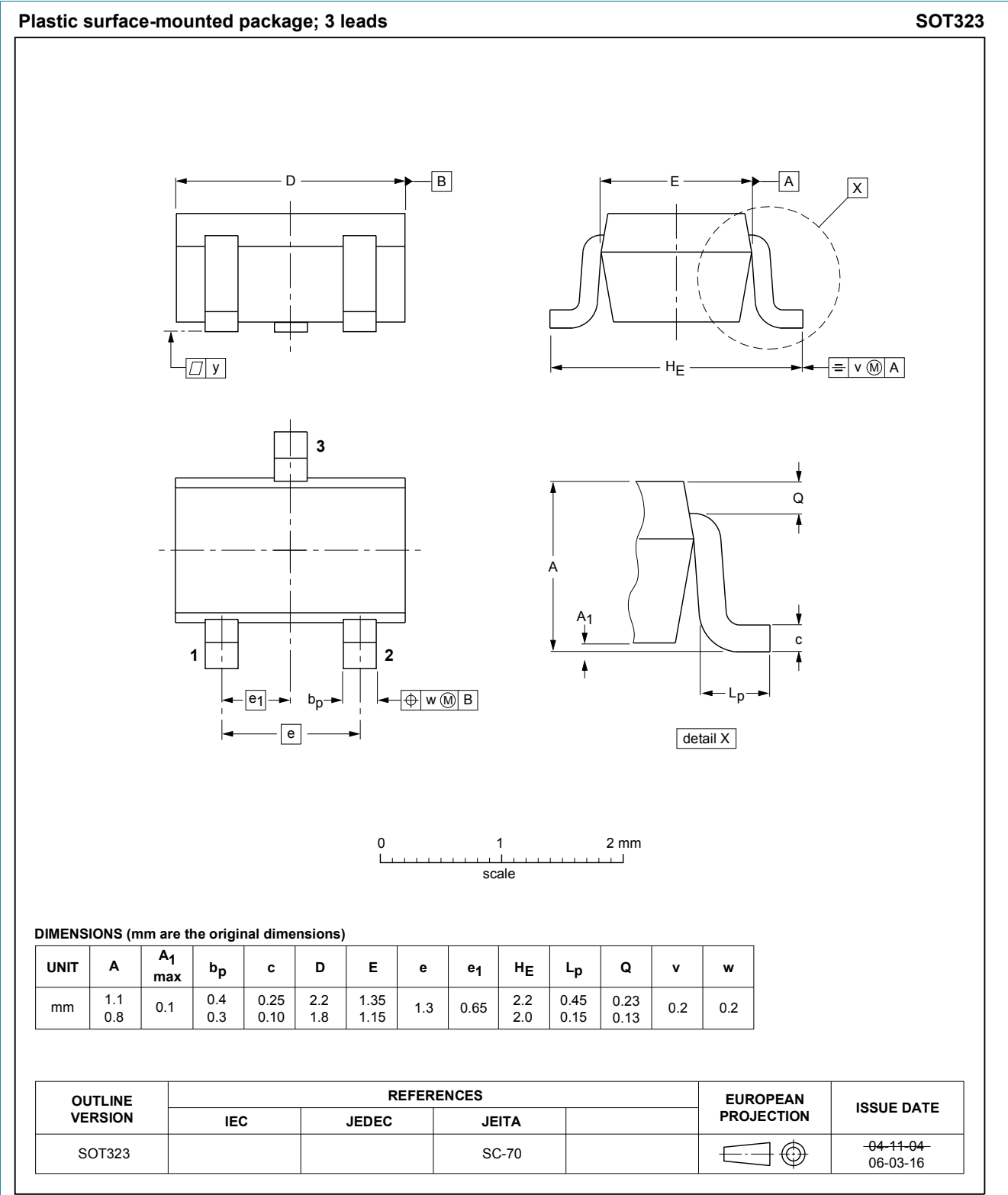
Figure 6. Package outline SOT323
