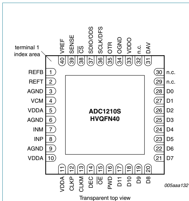
Fig 2. Pin configuration with CMOS digital outputs selected
