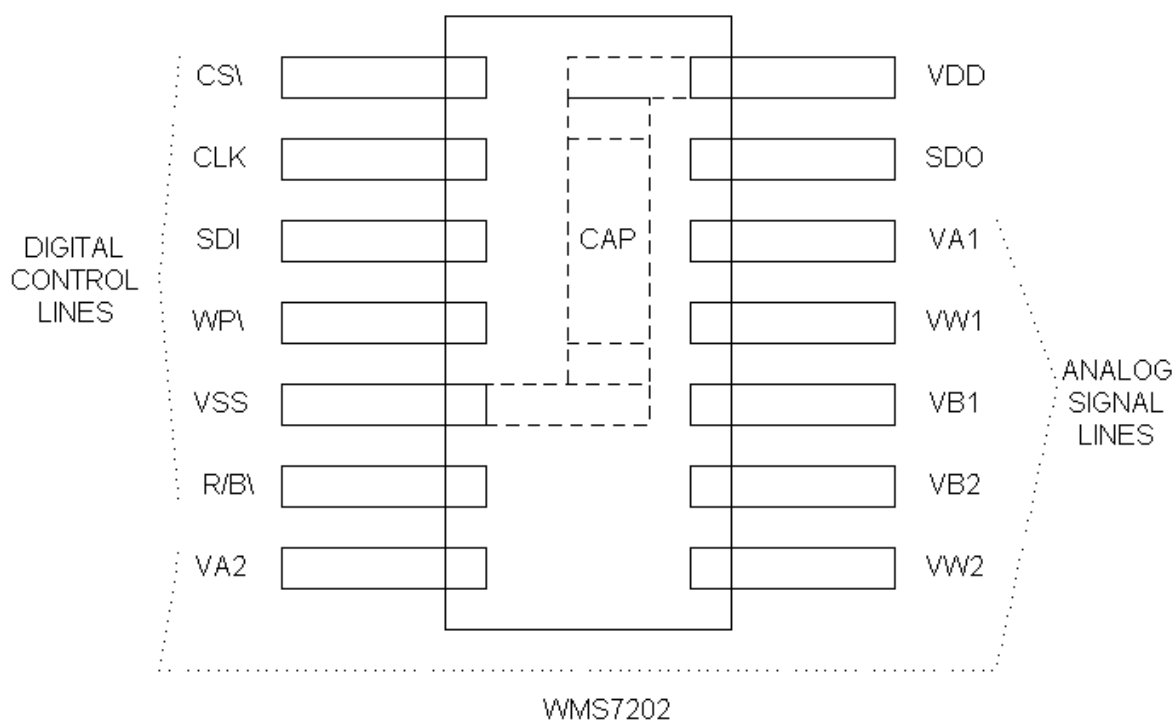
FIGURE 13 – WMS7202 LAYOUT
