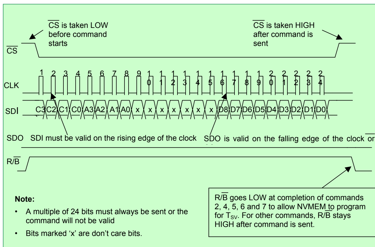
FIGURE 5 – SPI COMMAND WAVEFORMS
