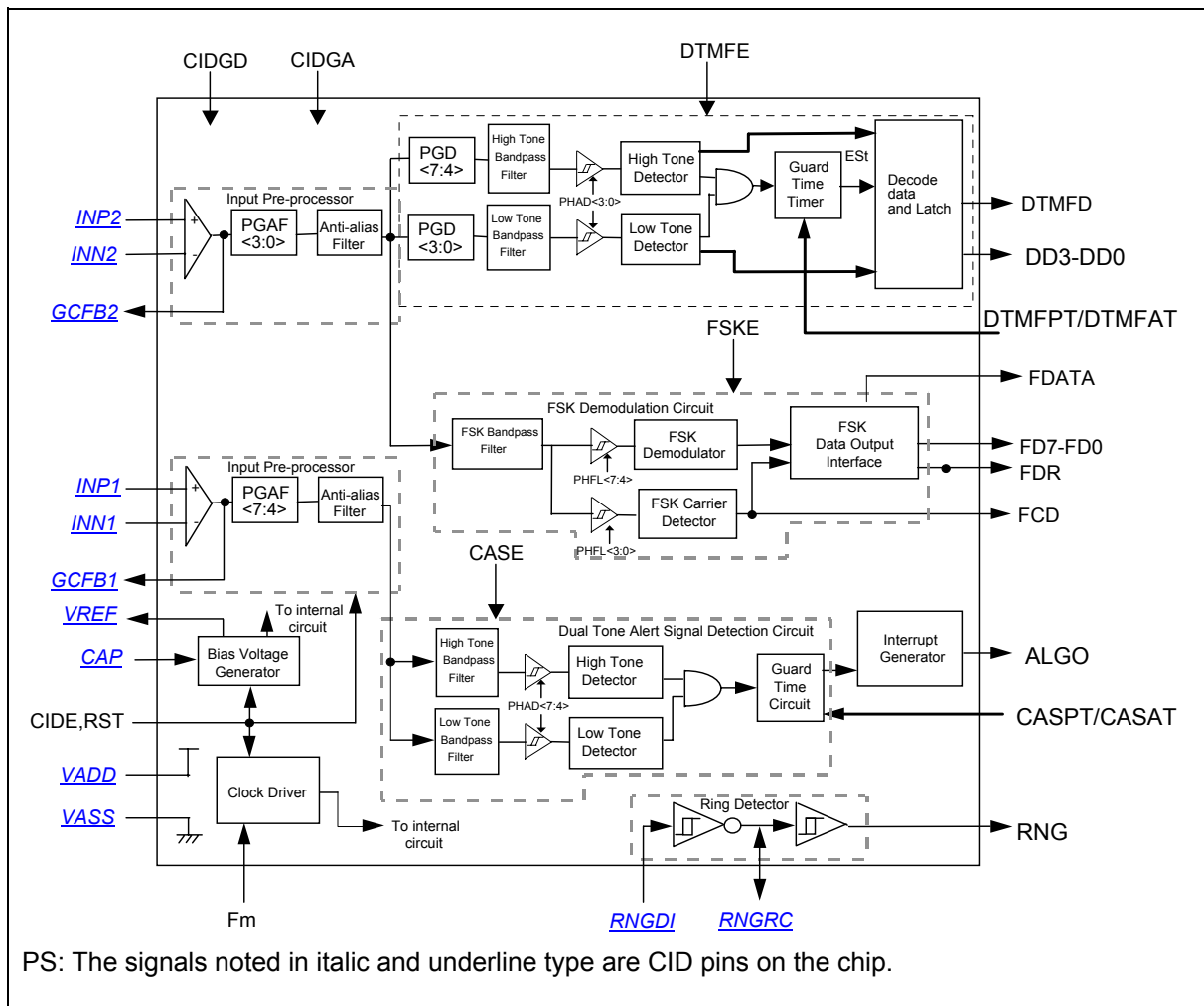
Figure 6-14 The CID Block Diagram
