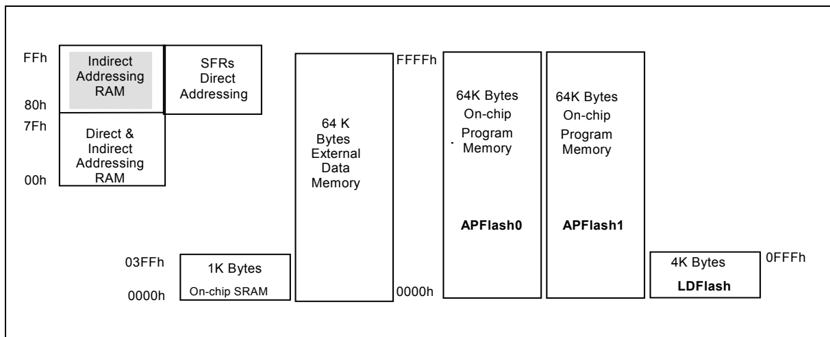
Figure 1. Memory Map
