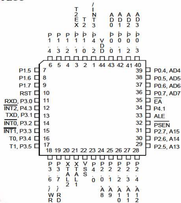
44-Pin PLCC
