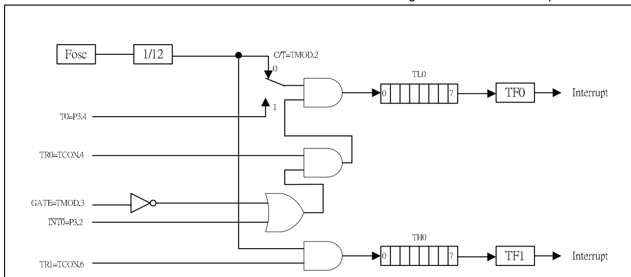
Figure 14- 3 Timer/Counter Mode 3
