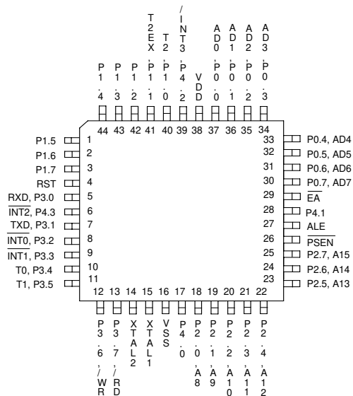
44-Pin QFP
