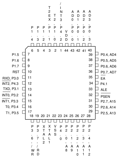
44-Pin PLCC
