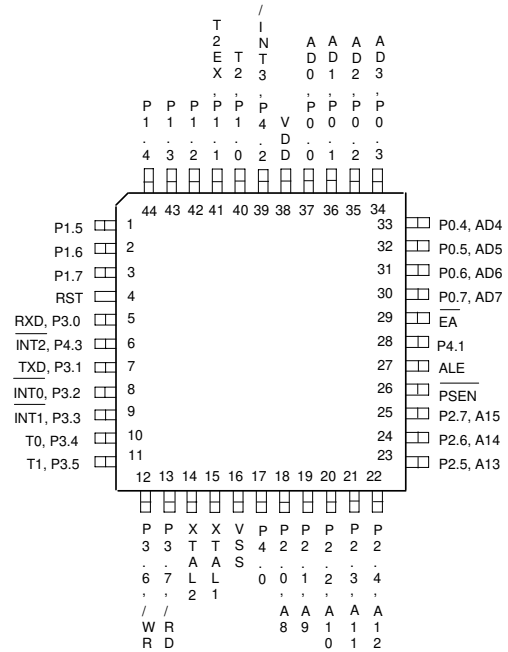
44-Pin QFP
