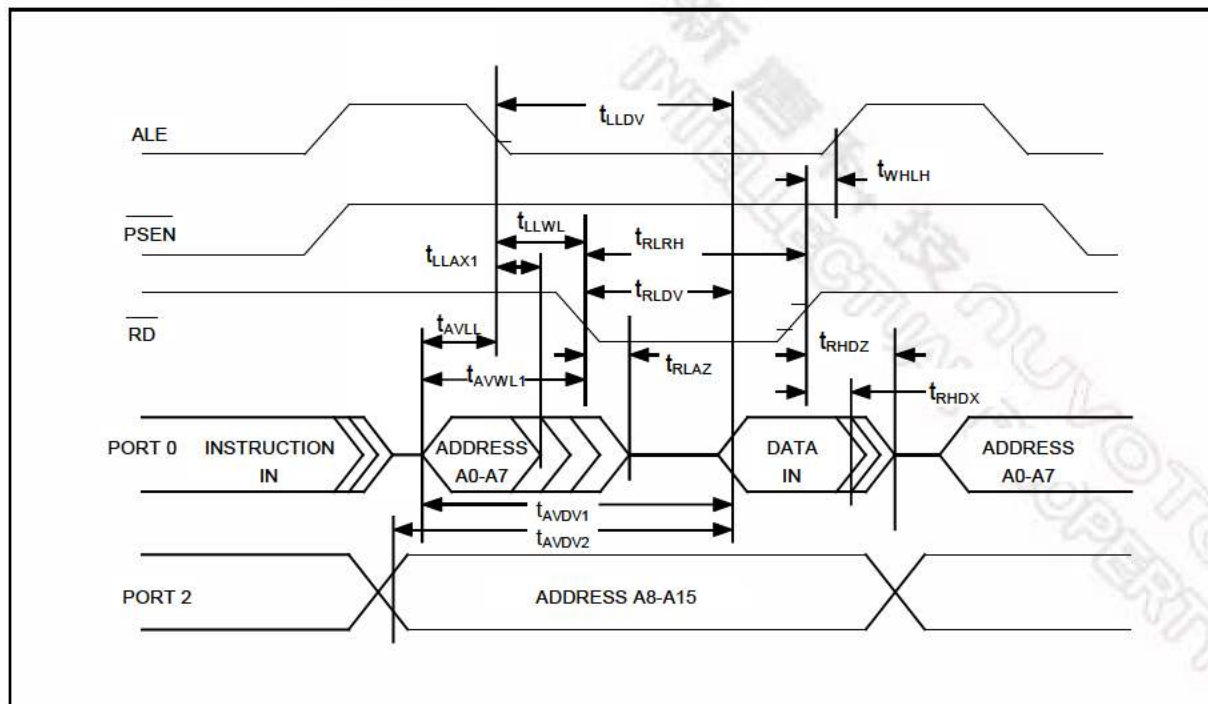
18.3.4 Data Memory Read Cycle
