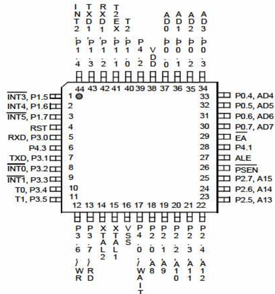
44-Pin QFP
