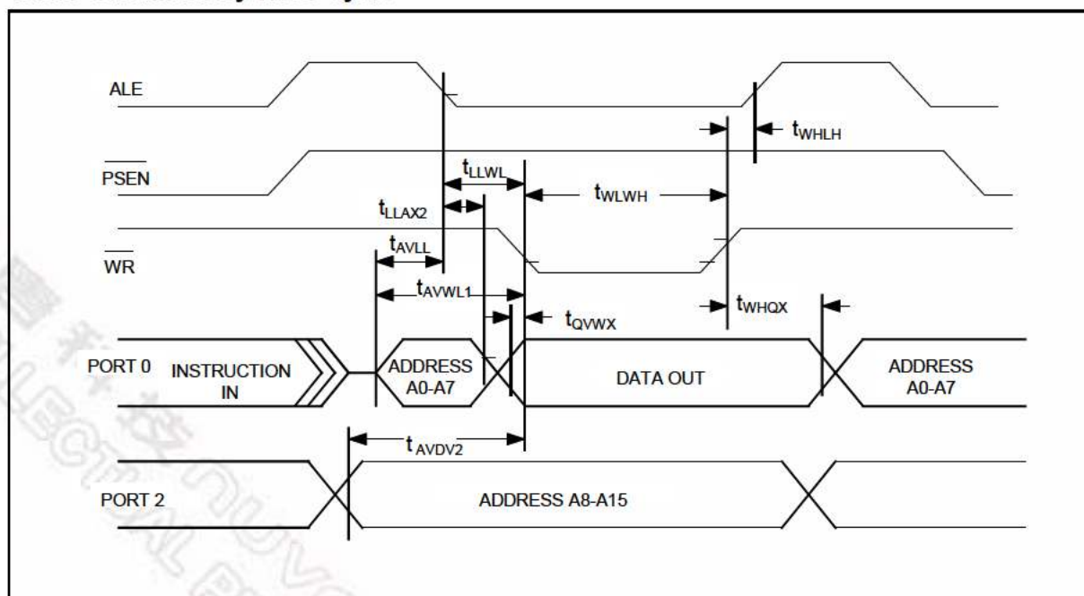
18.3.5 Data Memory Write Cycle
