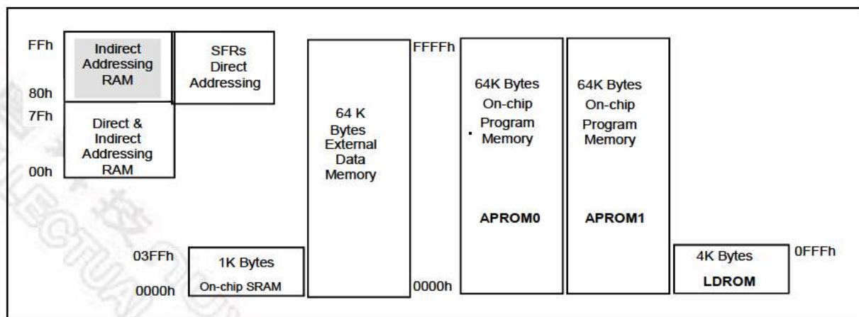
Figure 1. Memory Map
