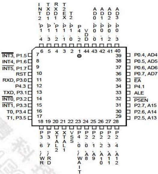
44-Pin PLCC
