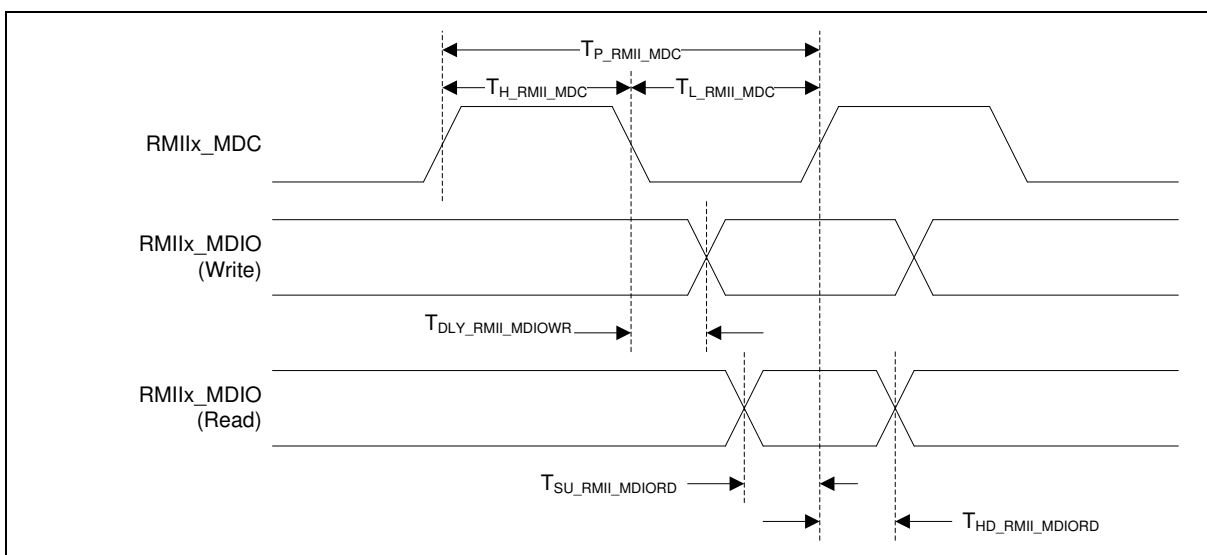
Figure 6.4-9 Ethernet PHY Management Interface Timing Diagram
