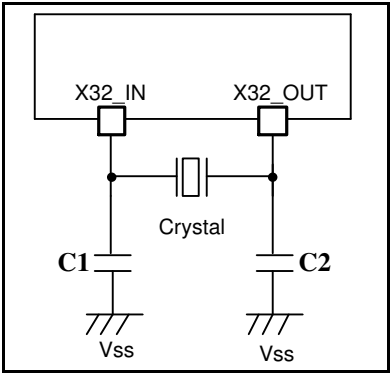
Figure 6.4-3 Typical LXT Crystal Application Circuit
