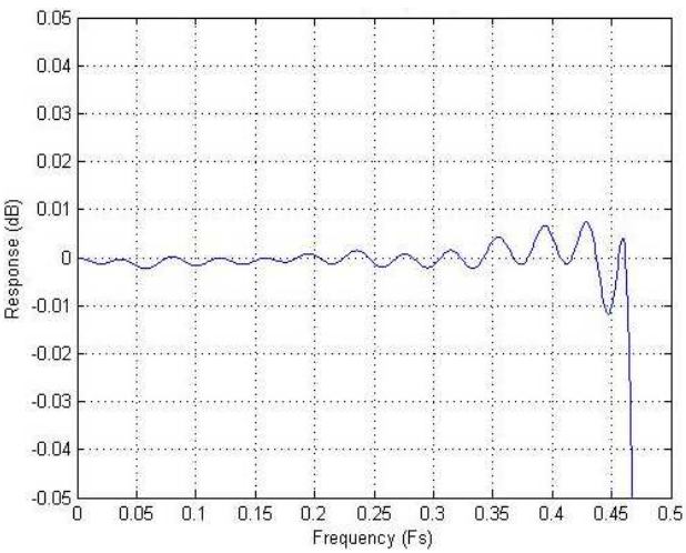
Figure 36: ADC Filter Ripple
