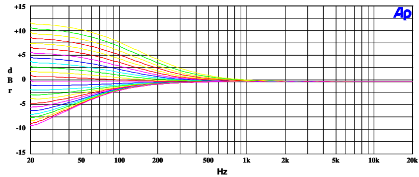
Figure 41: EQ Band 1 Gains for Lowest Cut-Off Frequency
