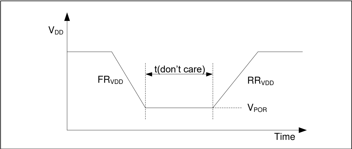
Figure 8-11 Power-up Ramp Condition
