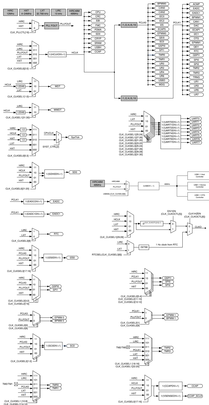
Figure 6-14 Clock Generator Global View Diagram (M48xGC/M48xE8)
