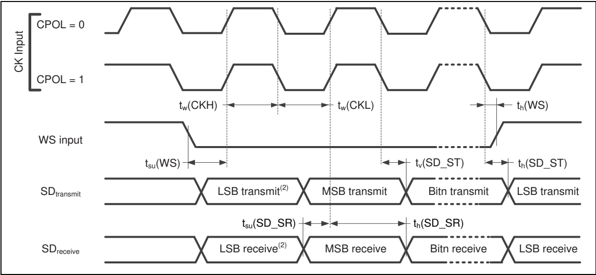
Figure 8-17 I²S Slave Mode Timing Diagram
