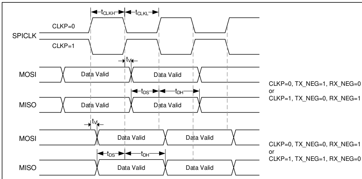
Figure 8-19 SPI Master Mode Timing Diagram
