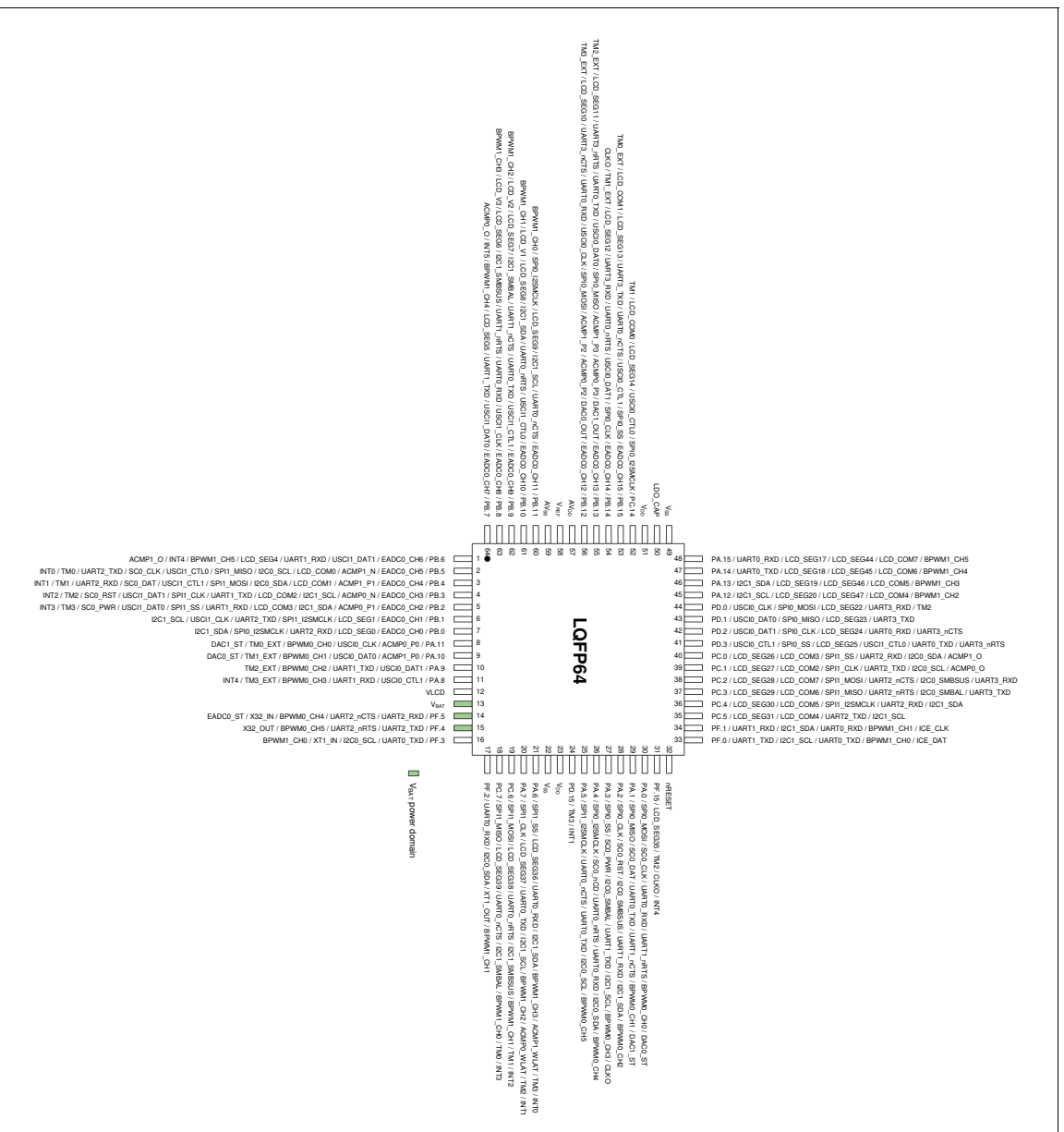
Figure 4.1-9 M254SG6AE Multi-function Pin Diagram
