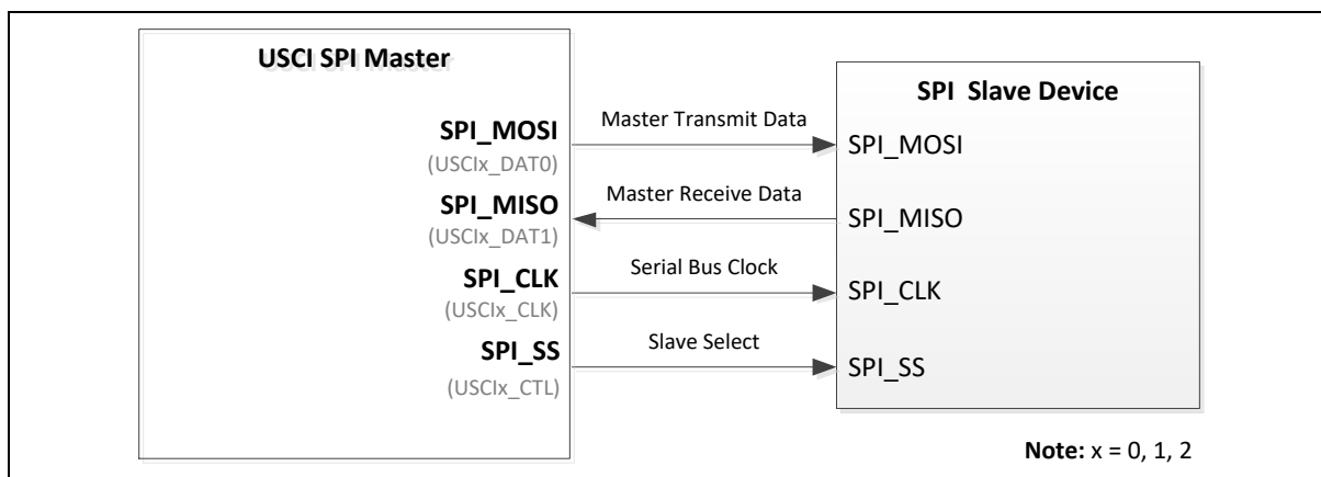
Figure 6.18-1 SPI Master Mode Application Block Diagram
