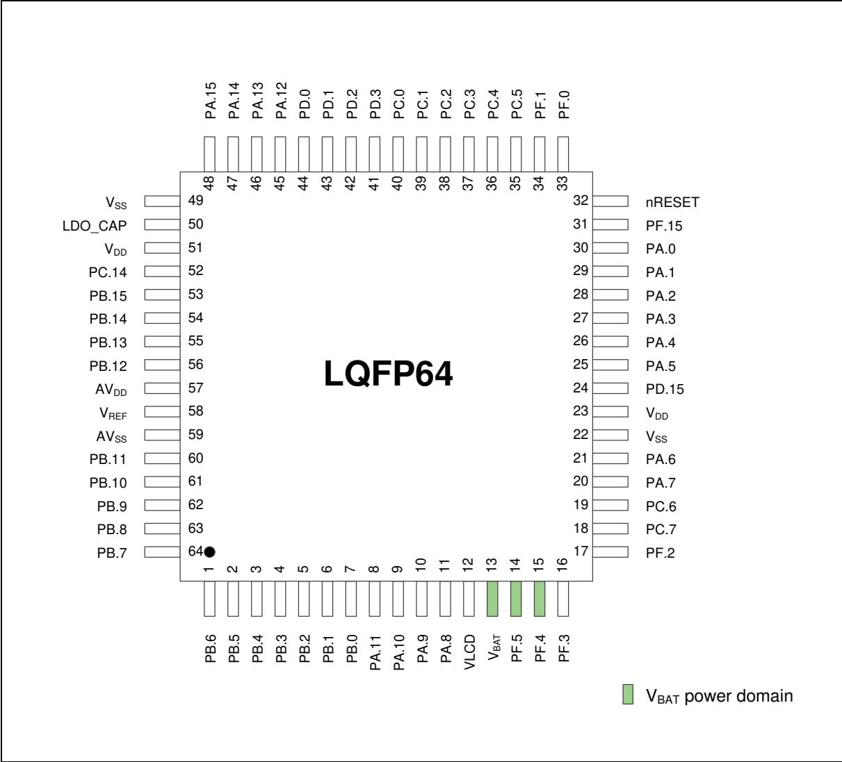
Figure 4.1-3 M254 Series LQFP 64-pin Diagram with V_{BAT}
