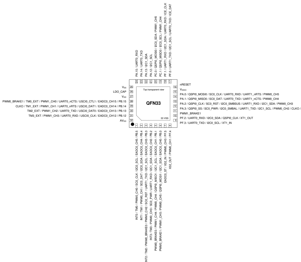
Figure 4.1-10 M251ZC2AE Multi-function Pin Diagram
