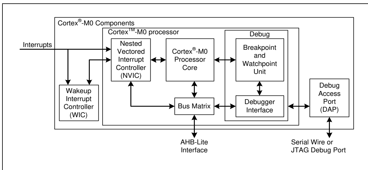
Figure 6.1-1 Functional Controller Diagram
