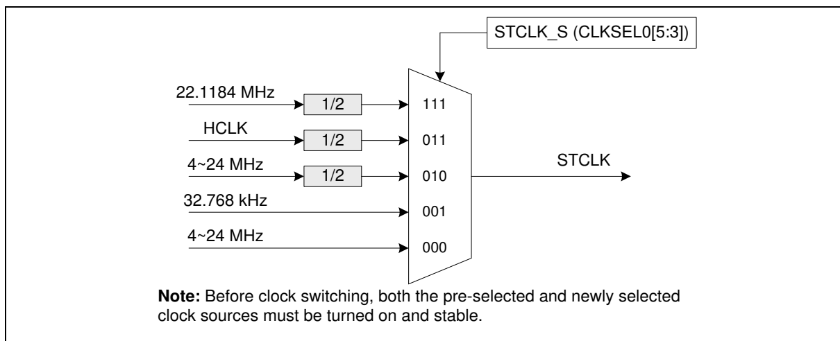
Figure 6.3-4 SysTick Clock Control Block Diagram
