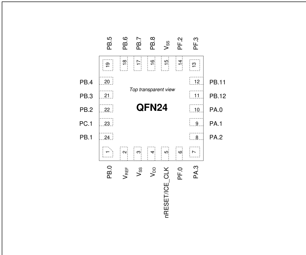
Figure 4.1-1 M029G/M030G/M031G Series QFN 24-pin Diagram
