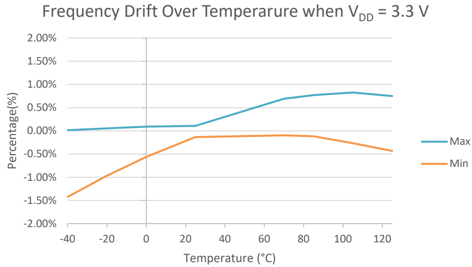
(b) Test Condition: V_{DD} = 3.3\text{ V} , Temp. = -40 \sim 125\text{ }^{\circ}\text{C}
