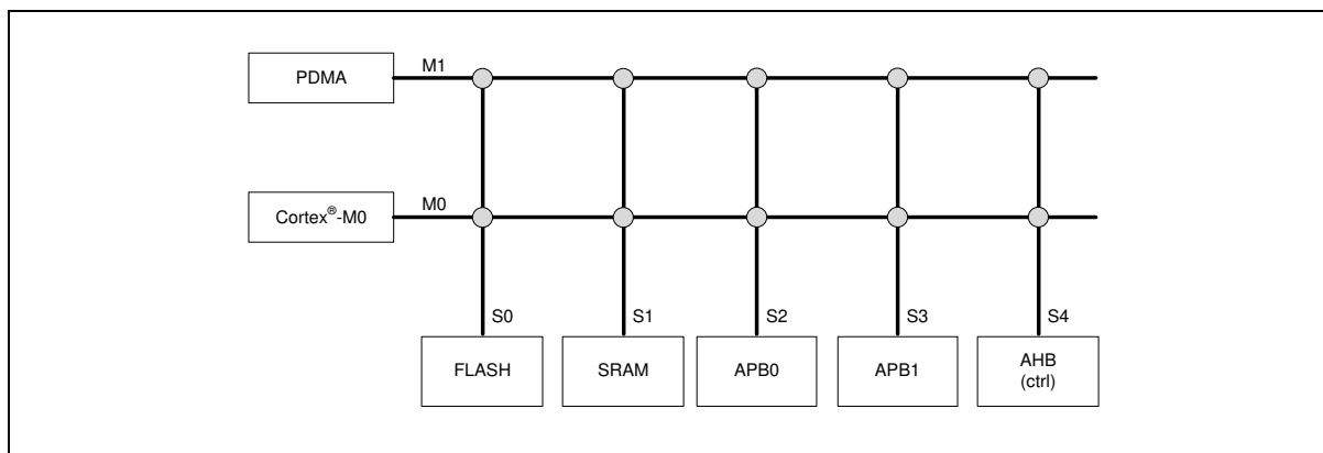
Figure 6.2-9 NuMicro® M029G/M030G/M031G Bus Matrix Diagram
