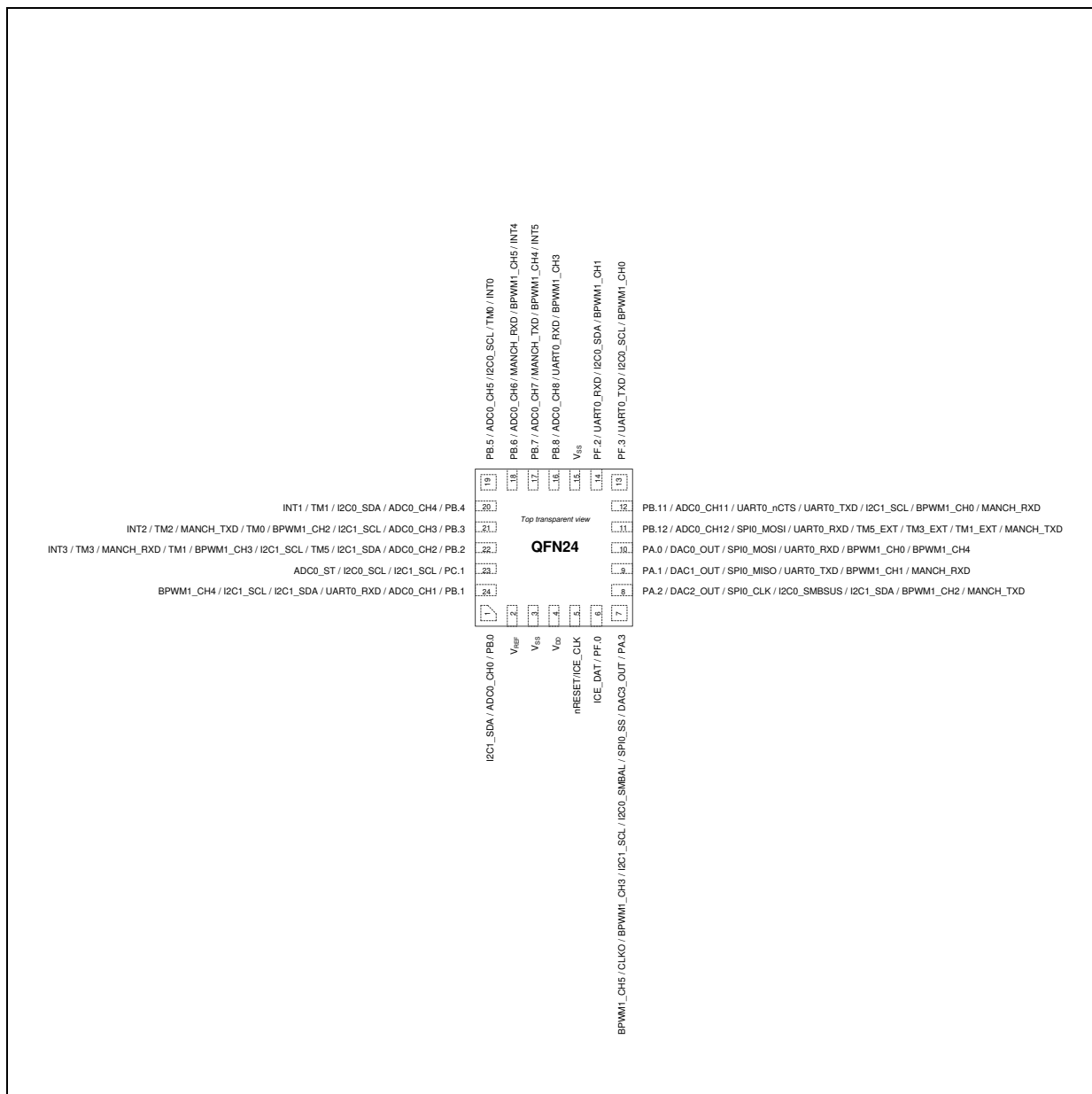
Figure 4.1-6 M031G Series QFN 24-pin Multi-function Pin Diagram
