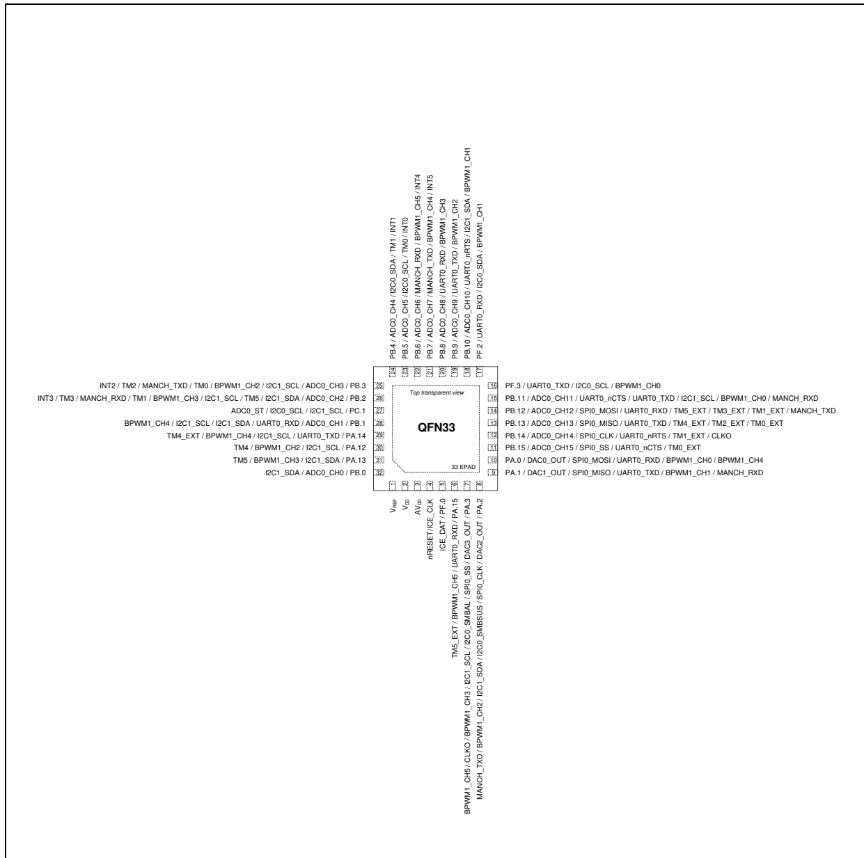
Figure 4.1-7 M031GTD2AE and M031GTC2AE Multi-function Pin Diagram
