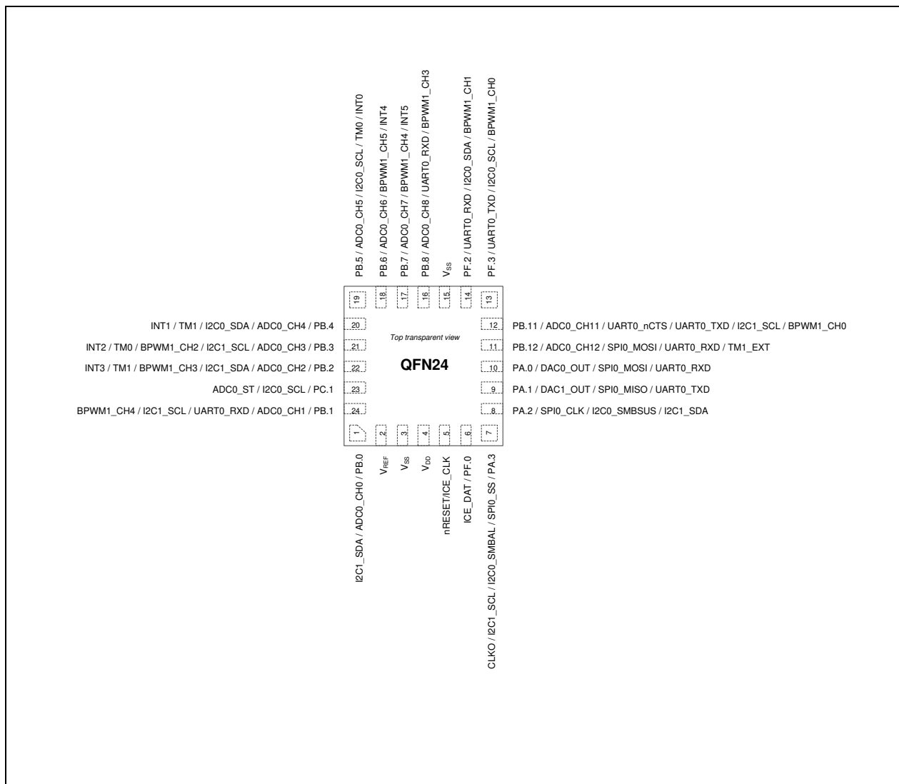
Figure 4.1-3 M029G Series QFN 24-pin Multi-function Pin Diagram
