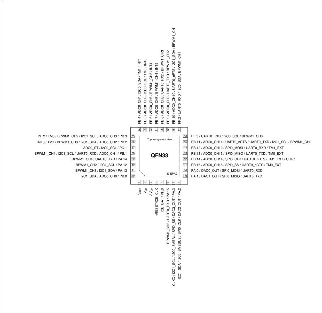
Figure 4.1-5 M030GTC1AE and M030GTD1AE Multi-function Pin Diagram
