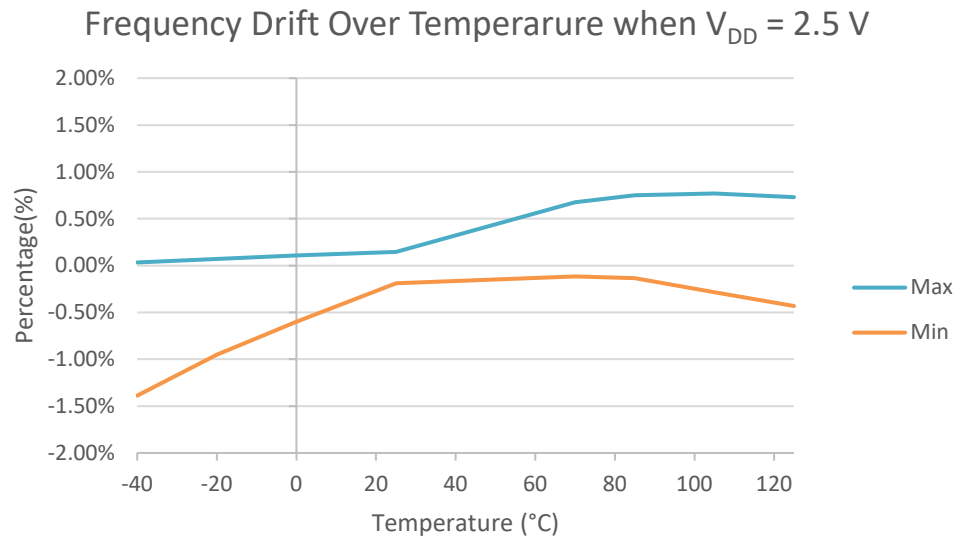
(c) Test Condition: V_{DD} = 2.5\text{ V} , Temp. = -40 \sim 125\text{ }^{\circ}\text{C}
