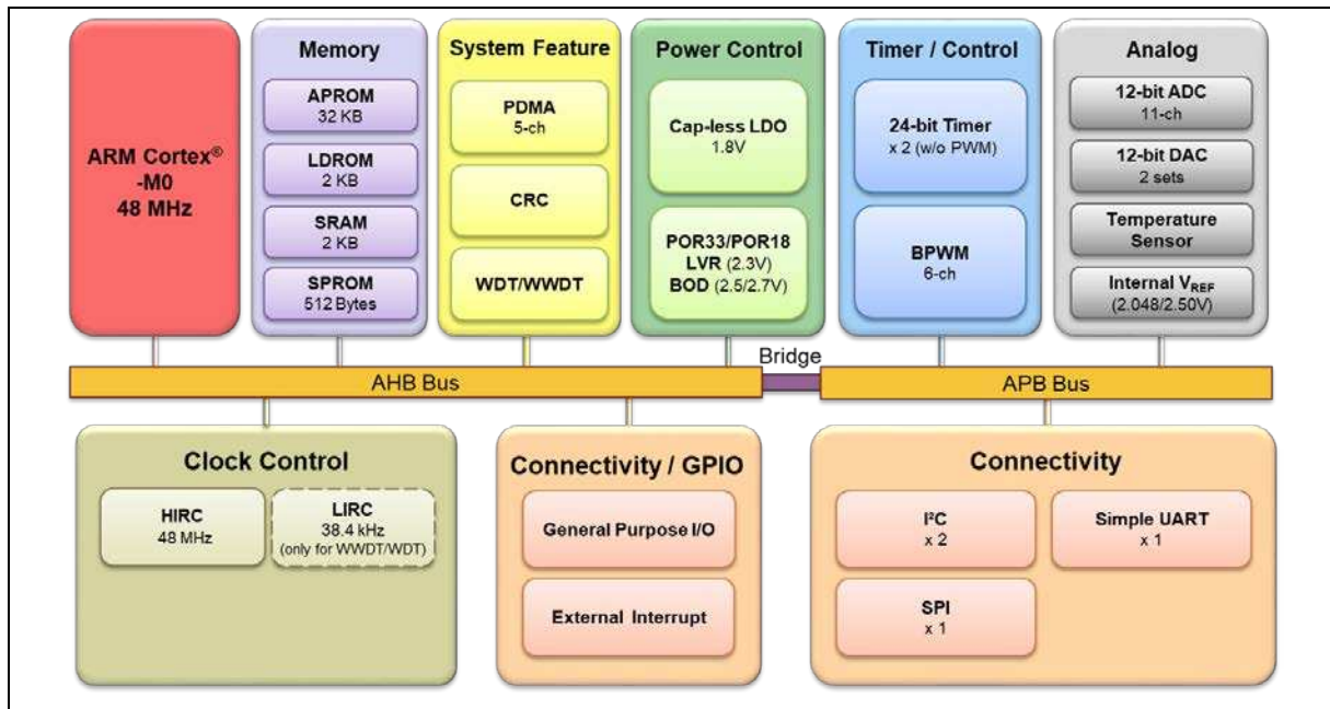
Figure 5-1 NuMicro M029G Block Diagram
