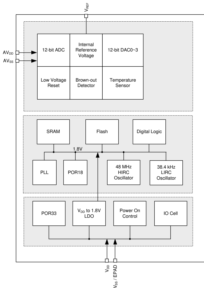
Figure 6.2-6 NuMicro® M029G/M030G/M031G Power Distribution Diagram
