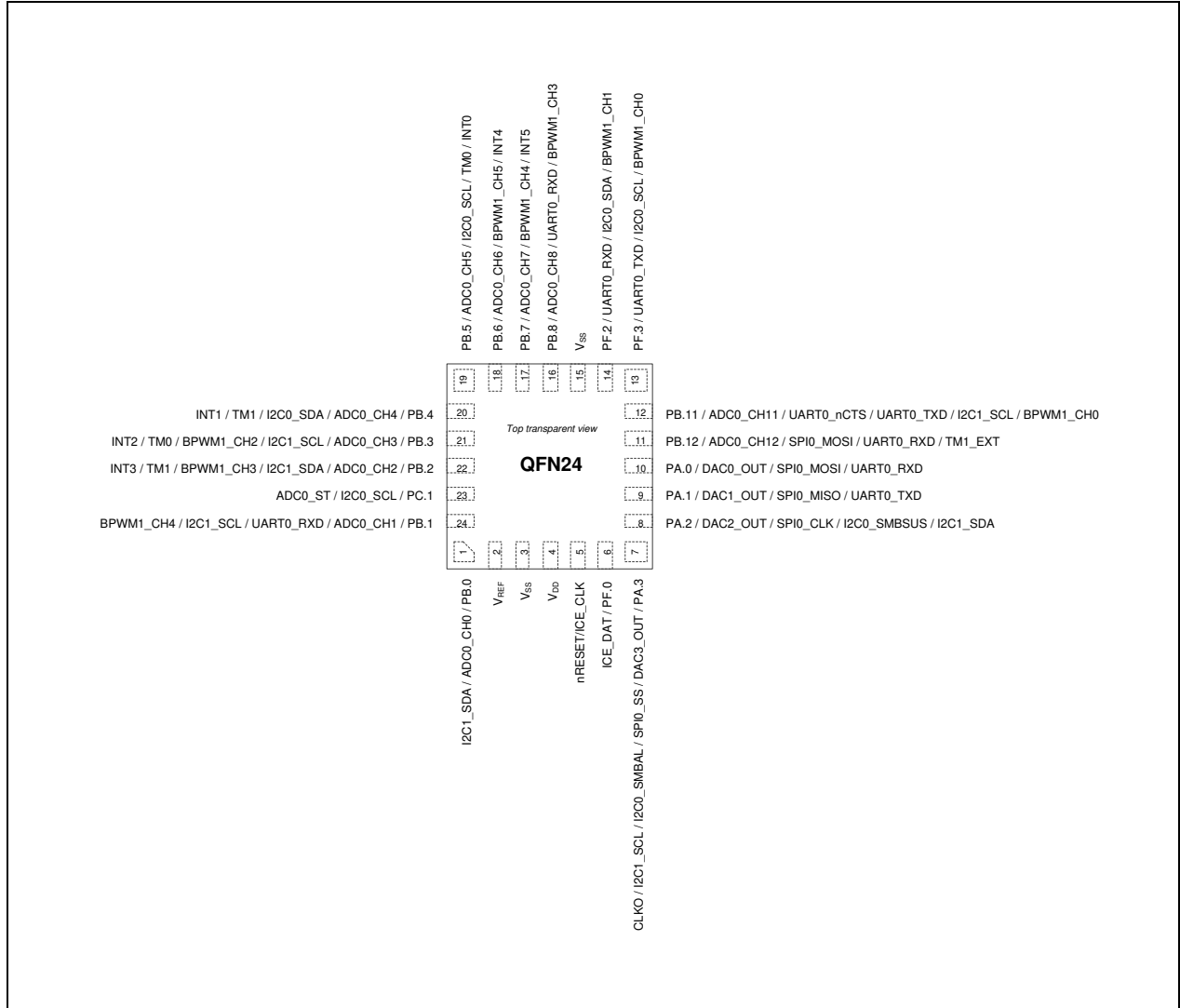
Figure 4.1-4 M030G Series QFN 24-pin Multi-function Pin Diagram
