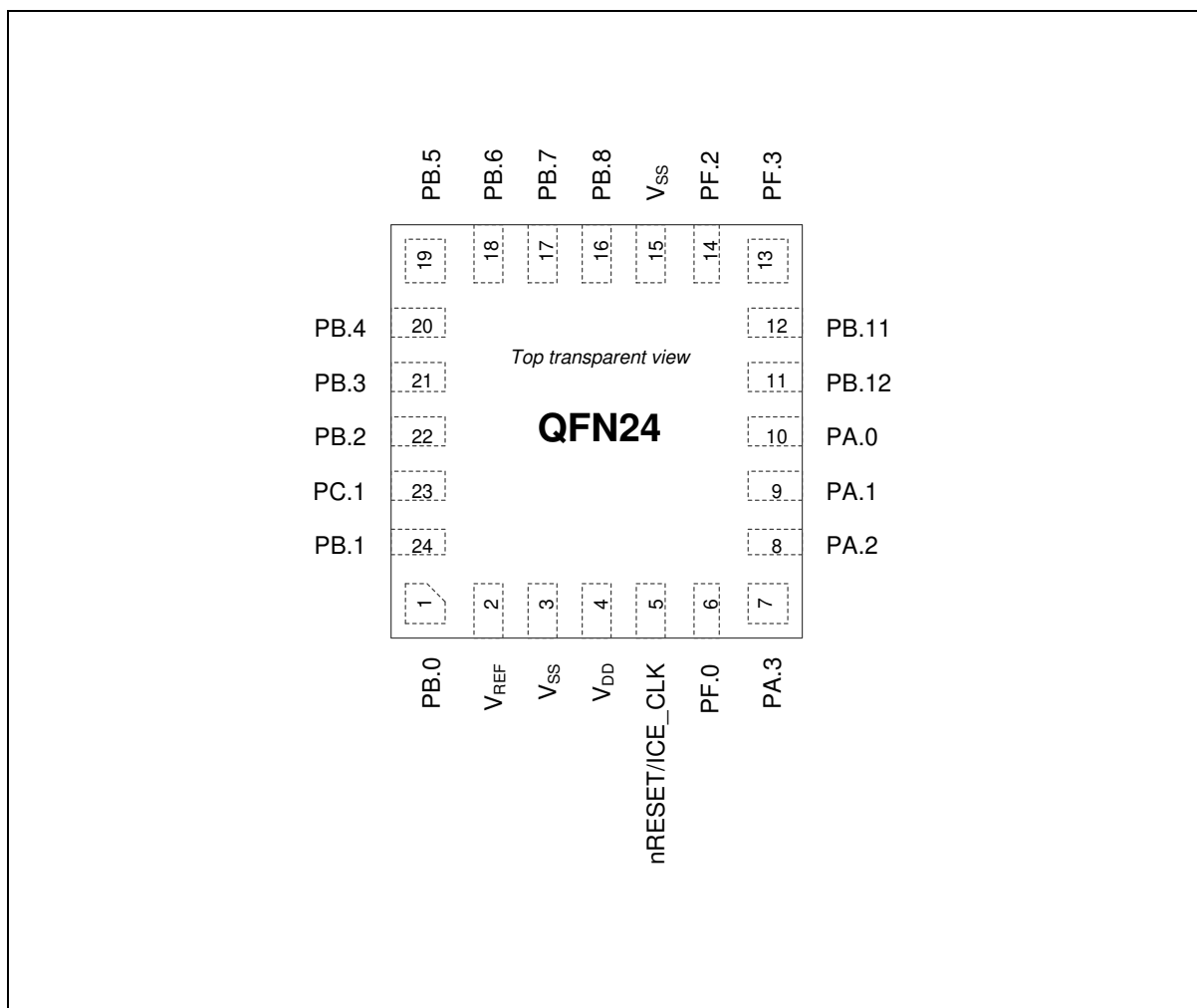
Figure 4.1-1 M029G/M030G/M031G Series QFN 24-pin Diagram
