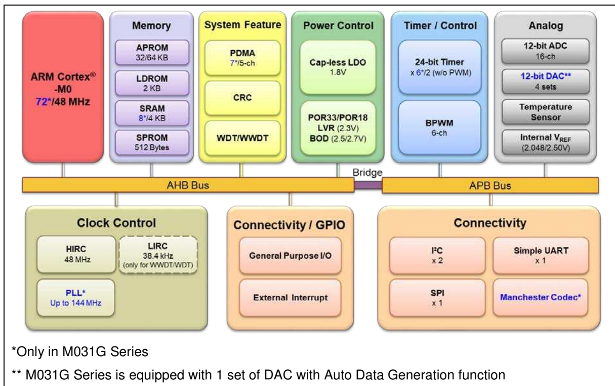
Figure 5-2 NuMicro M030G/M031G Block Diagram
