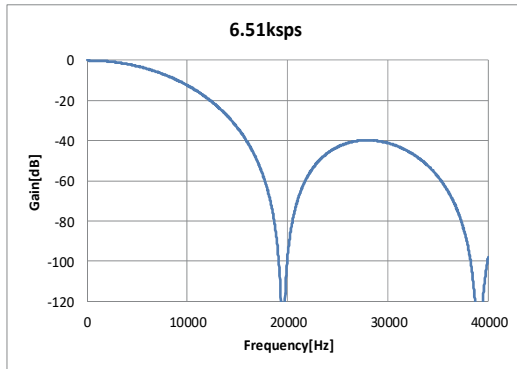
DR=6.51ksps
