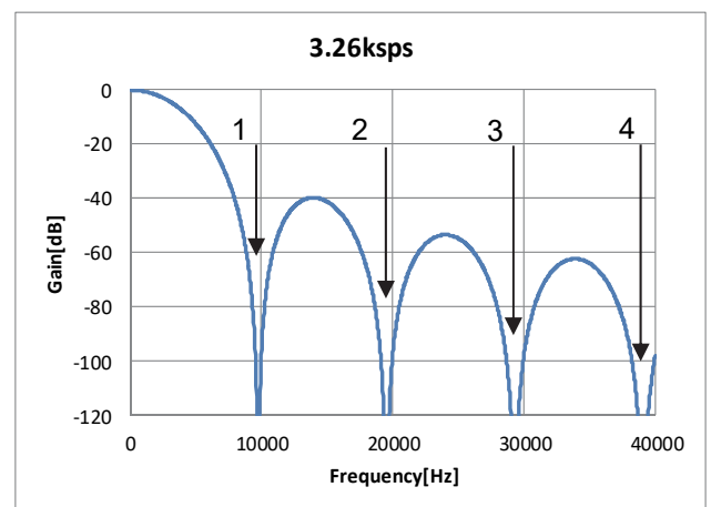
DR=3.26ksps
