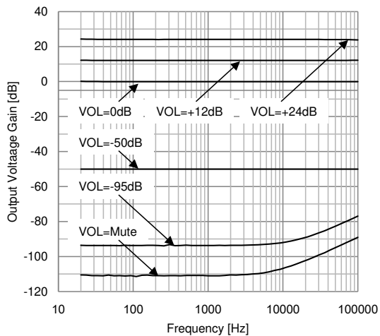
Output Voltage Gain vs Frequency V=±7V, Vin=2Vrms (VOL=0, -50, -95dB, Mute), Vin=0.1Vrms (VOL=+12, +24dB), Bandpass
