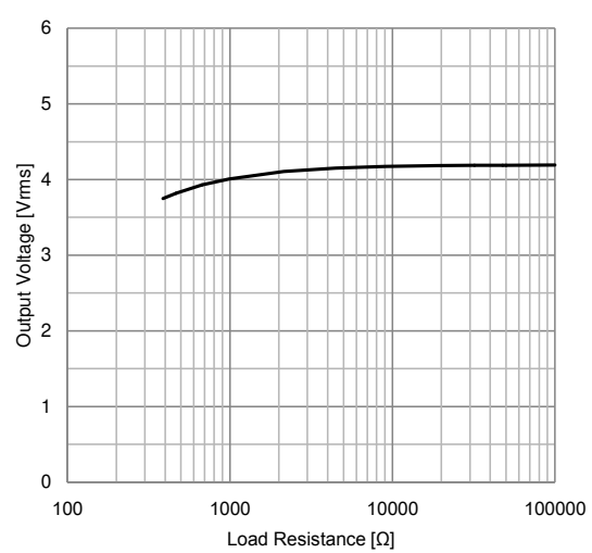
Output Voltage vs Load Resistance V=±7V, f=1kHz, Vin=4.2Vrms
