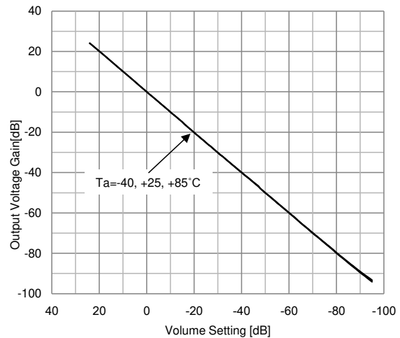
Output Voltage Gain vs Volume Setting V=±7V, Vin=2Vrms (VOL=0, -50, -95dB, Mute), Vin=0.1Vrms (VOL=+12, +24dB), Bandpass
