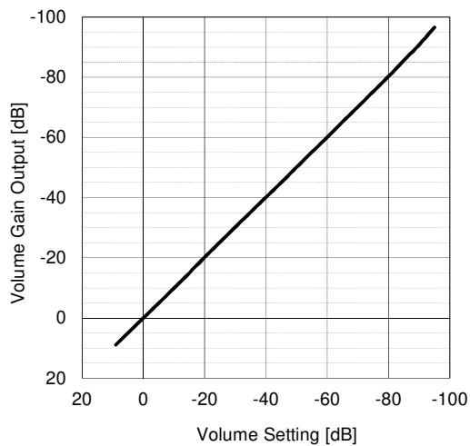
Volume Gain Output vs Volume Setting V^+=9V , T_a=25^\circ C , f=1kHz , Bandpass
