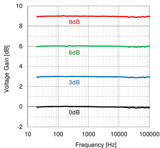
Voltage Gain Output vs Frequency V^+=9V , T_a=25^\circ C , V_{in}=0.1V_{rms} , Bandpass
