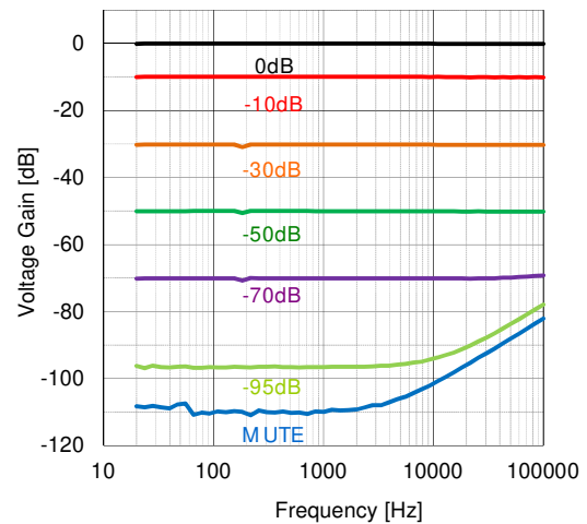
Voltage Gain Output vs Frequency V^+=9V , T_a=25^\circ C , V_{in}=1.5V_{rms} , Bandpass
