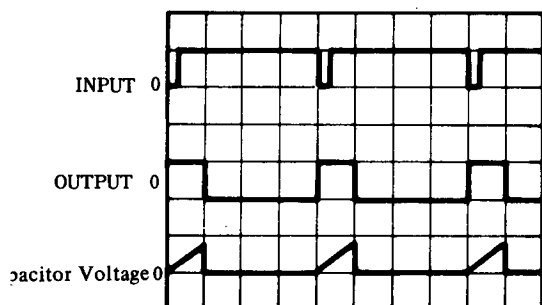
Fig.2 Wave Form
