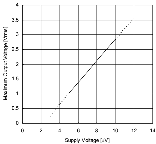
Maximum Output Voltage vs Supply Voltage THD=1%, I/O: INA1-Aout
