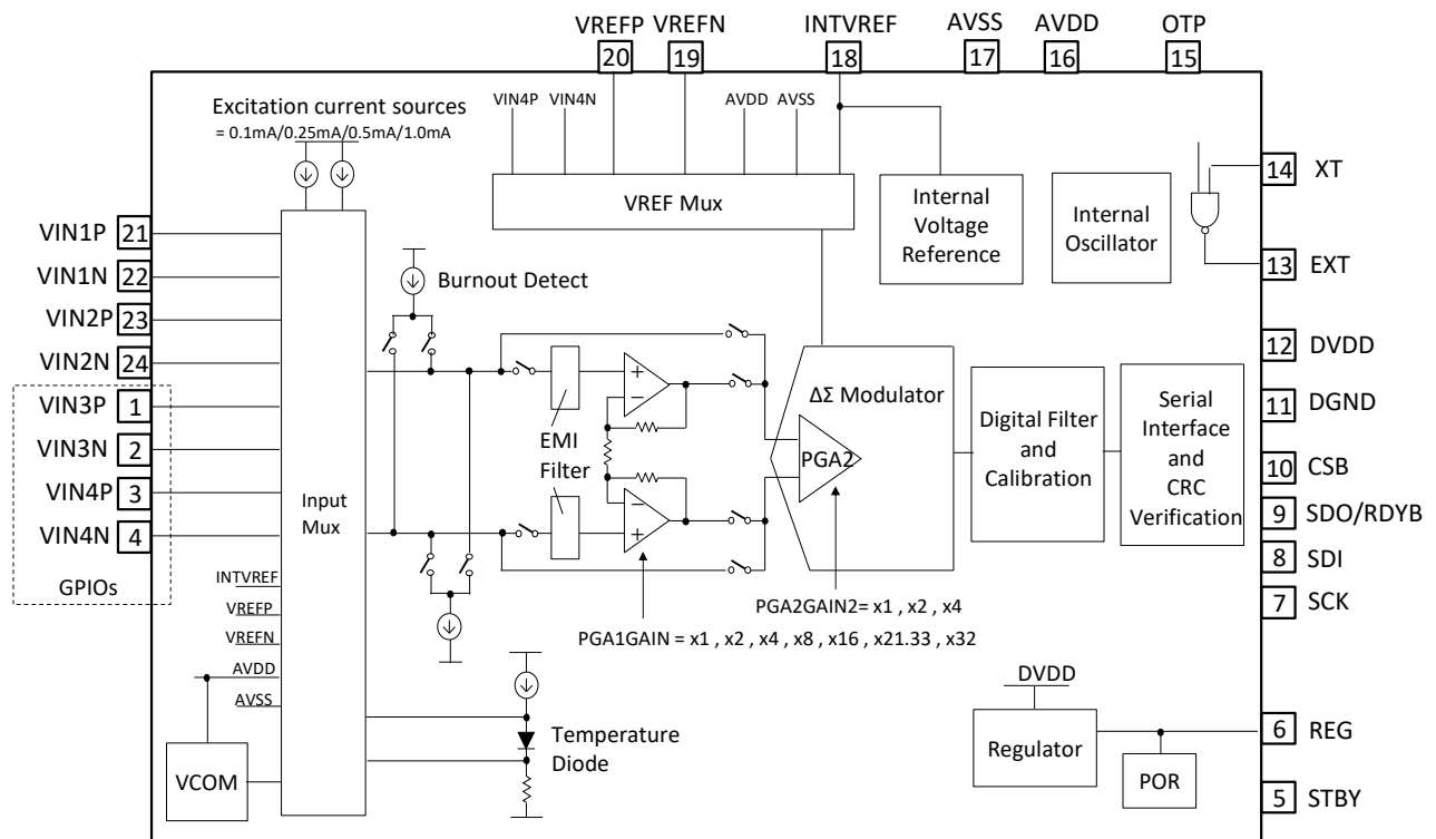
NA2202/2203/2204 Block Diagram
