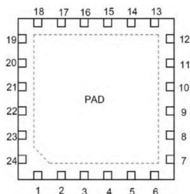
QFN4040-24-NB Pin Configuration
