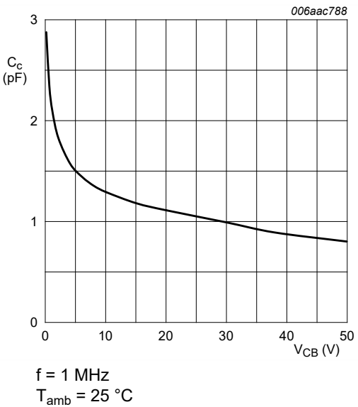
Fig. 8. TR1 (NPN): Collector capacitance as a function of collector-base voltage; typical values
