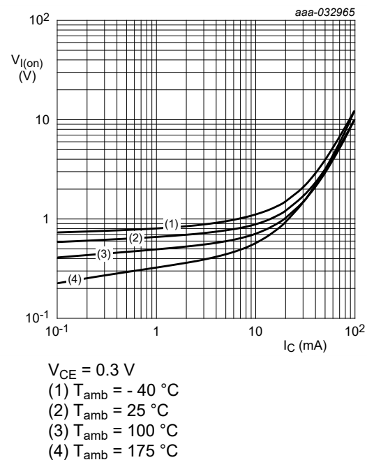
Fig. 6. TR1 (NPN): On-state input voltage as a function of collector current; typical values
