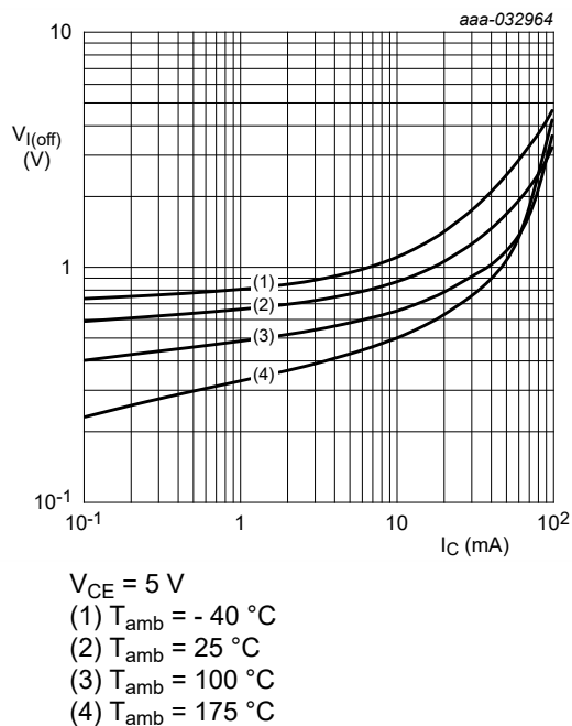
Fig. 5. TR1 (NPN): Off-state input voltage as a function of collector current; typical values
