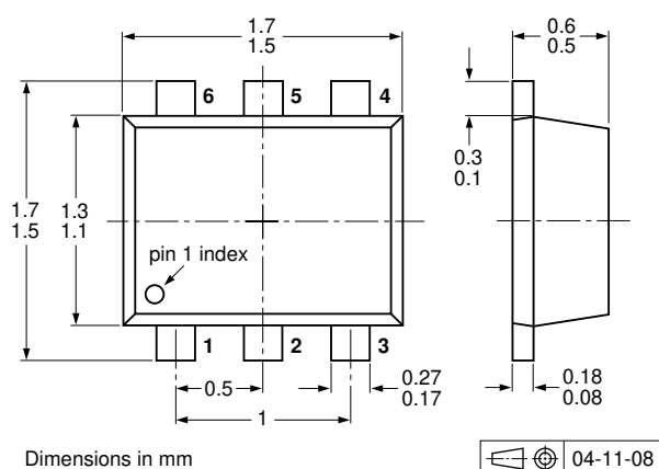
Fig 16. Package outline PEMD13 (SOT666)
