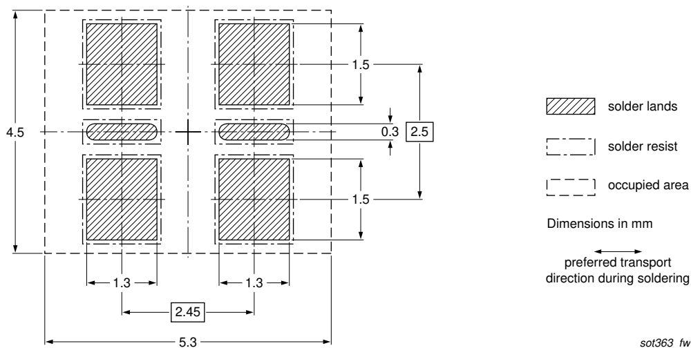
Fig 20. Wave soldering footprint PUMD12 (SOT363)
