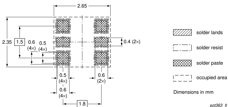
Fig 19. Reflow soldering footprint PUMD12 (SOT363)
