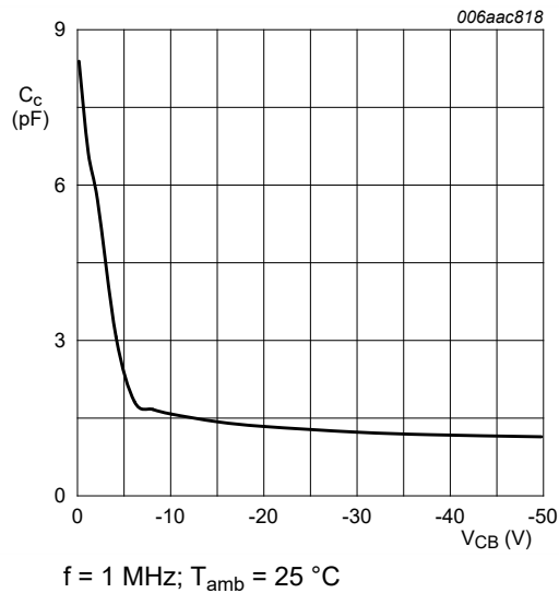
Fig. 14. PNP transistor: Collector capacitance as a function of collector-base voltage; typical values
