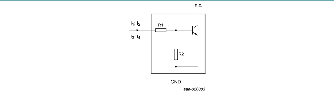
Fig. 17. PNP transistor: Resistor test circuit
