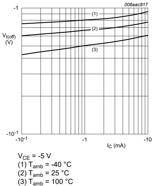
Fig. 13. PNP transistor: Off-state input voltage as a function of collector current; typical values
