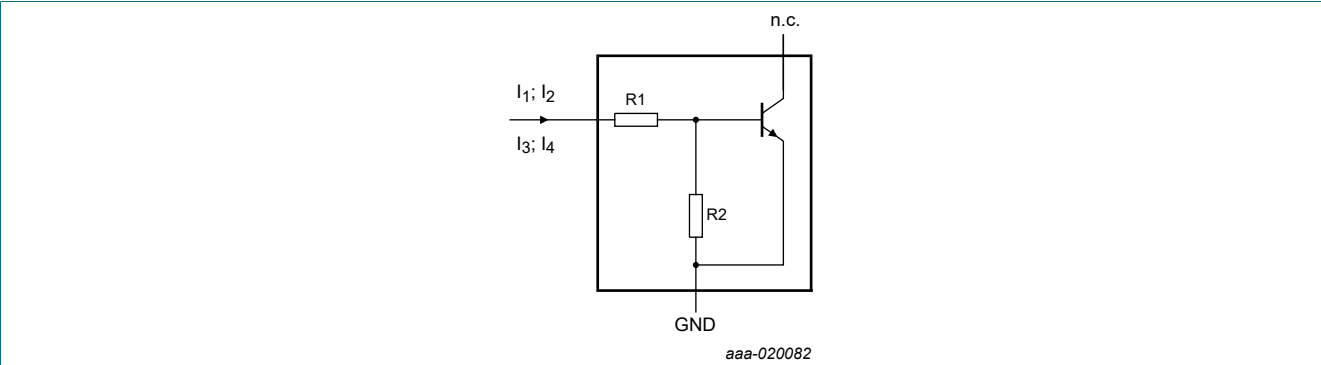
Fig. 16. NPN transistor: Resistor test circuit
