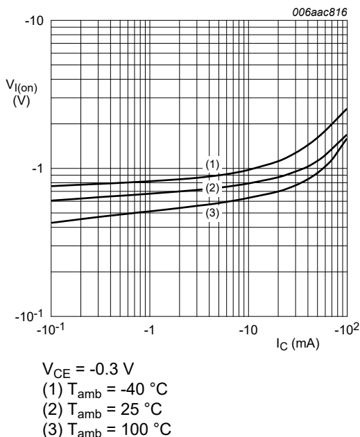
Fig. 12. PNP transistor: On-state input voltage as a function of collector current; typical values
